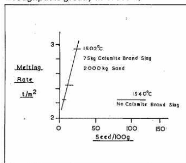
Fig 2. Graph showing the benefits from the introduction of Calumite brand slag to a flint glass furnace. (Better refining and lower furnace temperatures even when throughput is greatly increased.)
