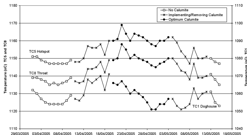
Figure 1. The effects of Calumite addition on furnace bottom temperatures. Daily spot temperature readings taken at 7 am
